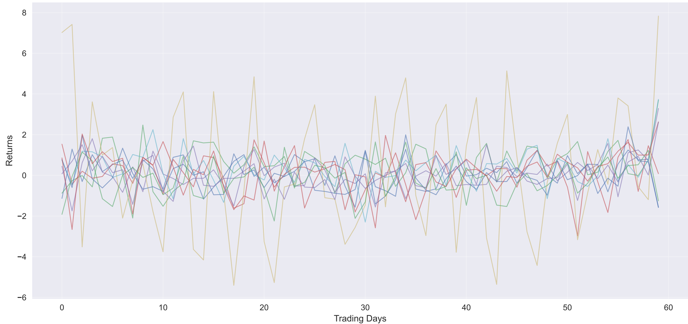
Zero Conditioned: Sample Paths (First 10)
